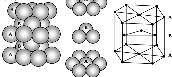
Fig. 5.9. Hexagonal close packing (hcp) in three
